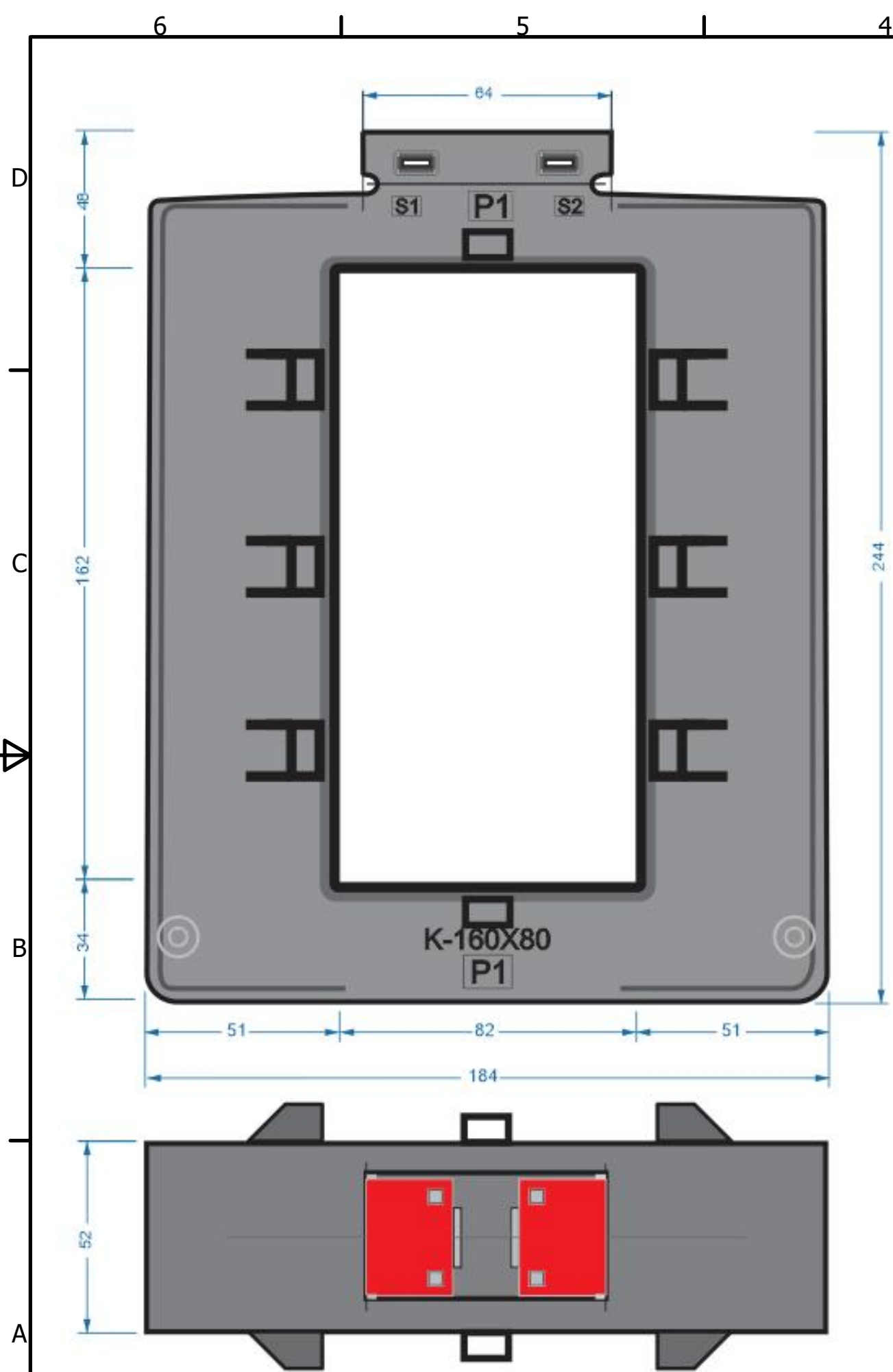
JP-816 Dimension Unit: mm
